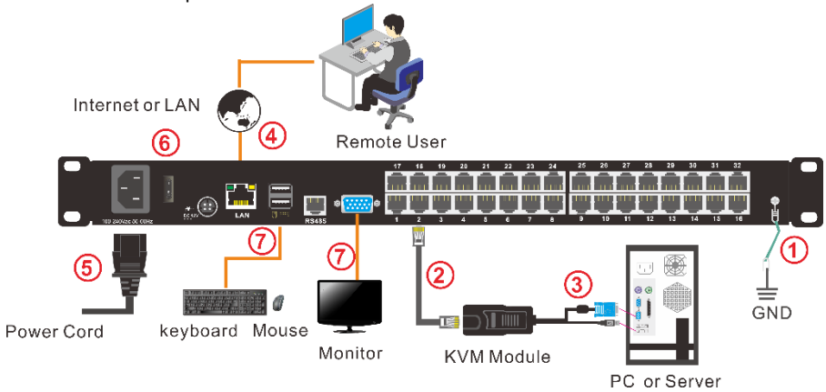
Figure 2.2 Installation diagram
