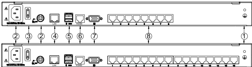
Figure 1.2 Rear view
