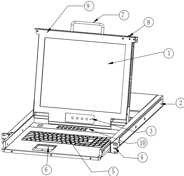
Figure 1.1 Front view
